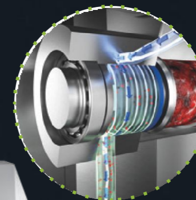
THE FLUSHING CHAMBER
